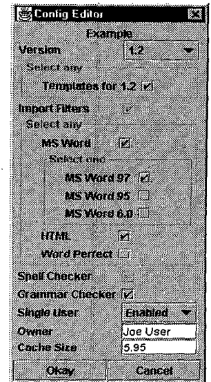
Figure 2: Configuration Editor
