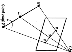
Figure 2.7. Illustration of 1D calibration objects.
