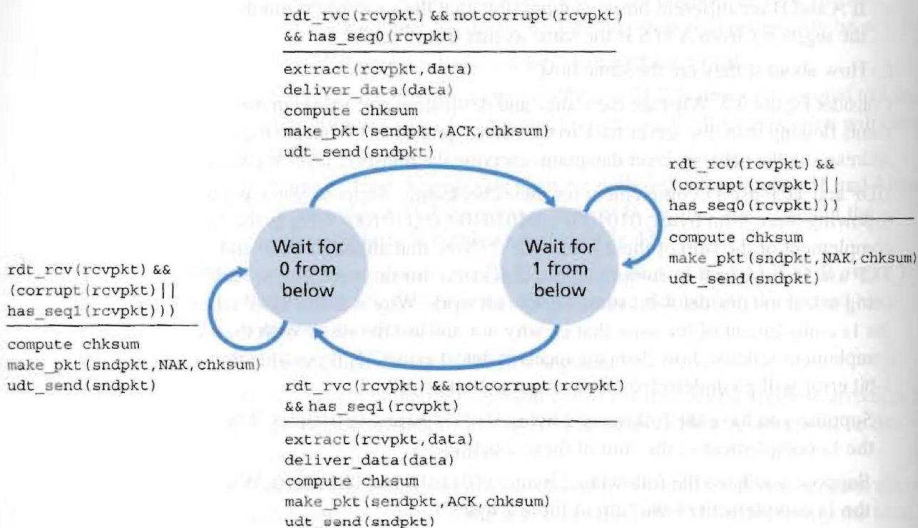
Figure 3.57 ♦ An incorrect receiver for protocol rdt 2.1
