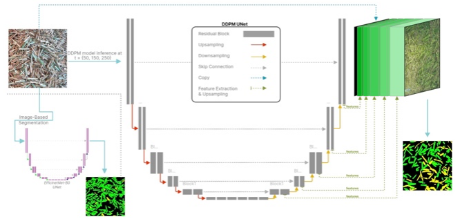
Fig. 6. DDPM and ControlNet-Based Diffusion Model
