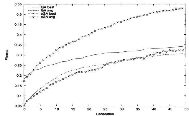
Figure 4: Comparison of the average fitness and best fitness for a population size of 500. Despite the difference in fitness of the best individual, the average fitness for the GA and cGA follow a very similar evolution.
