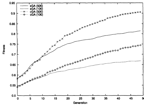
Figure 3: The even 5-parity problem for population size of 100 and 500. For this problem too the cGA outperforms the GA.
