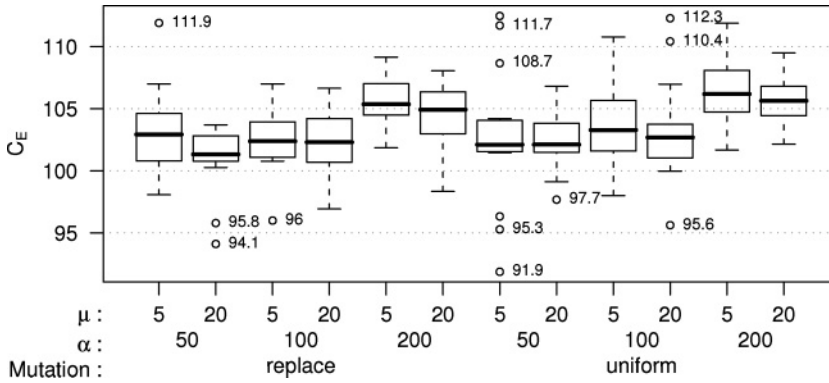
Figure 14: Boxplot of SEA results using level-controlled triggers (the Richmond network). The y axis gives the electricity cost ( C_E ). The x axis denotes all possible combinations of parameter mutation, population size ( \alpha ), and parent/offspring population size ( \mu ) used in the runs summarised by each boxplot.
