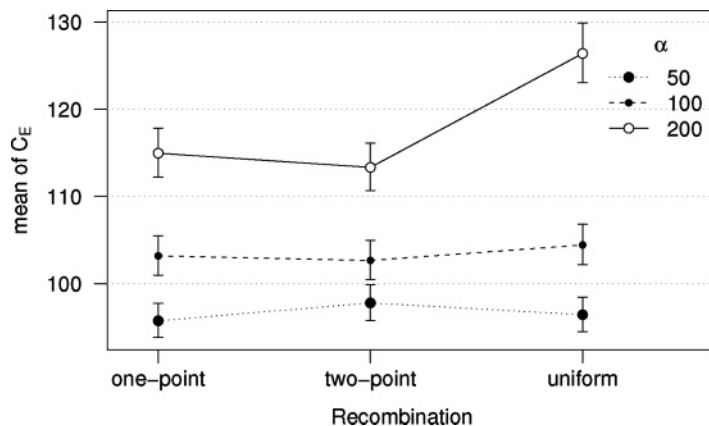
Figure 13: Interaction plot of SEA using the binary representation (the Richmond network). The y axis gives the electricity cost ( C_E ). The x axis gives different recombinations. Points joined with a line denote runs using the same population size ( \alpha ).
