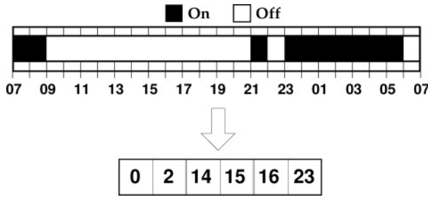
Figure 4: Example of absolute time-controlled trigger representation.
