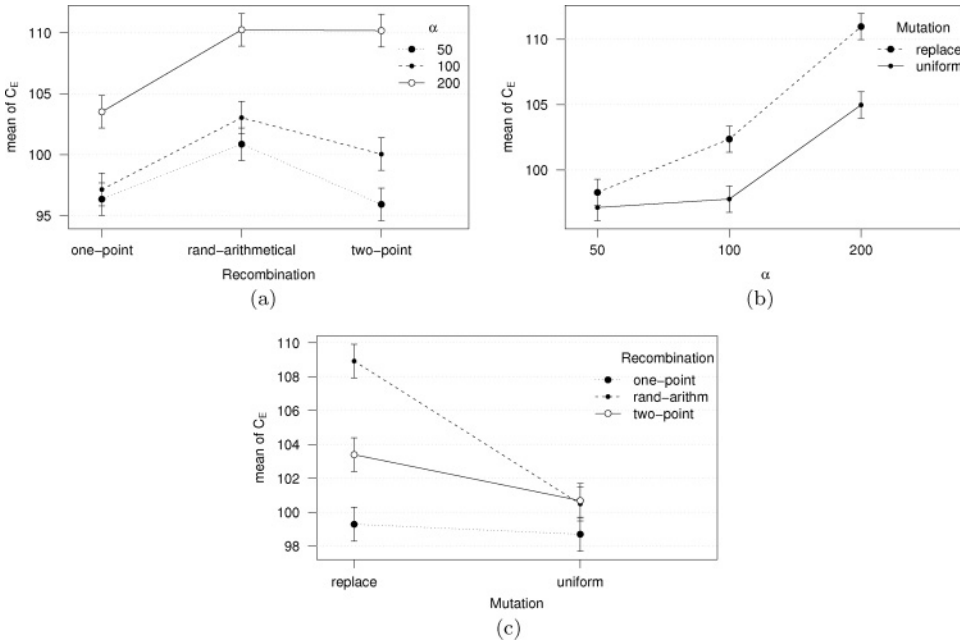
Figure 16: Interaction plots of SEA using absolute time-controlled triggers (the Richmond network). (a) Interaction between recombination operator and population size ( \alpha ). (b) Interaction between population size ( \alpha ) and mutation operator. (c) Interaction between mutation and recombination operators. The y axis gives the electricity cost ( C_E )
