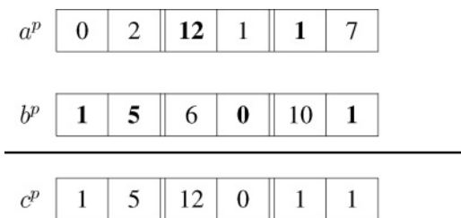
Figure 8: Example of uniform recombination for relative time-controlled trigger representation.
