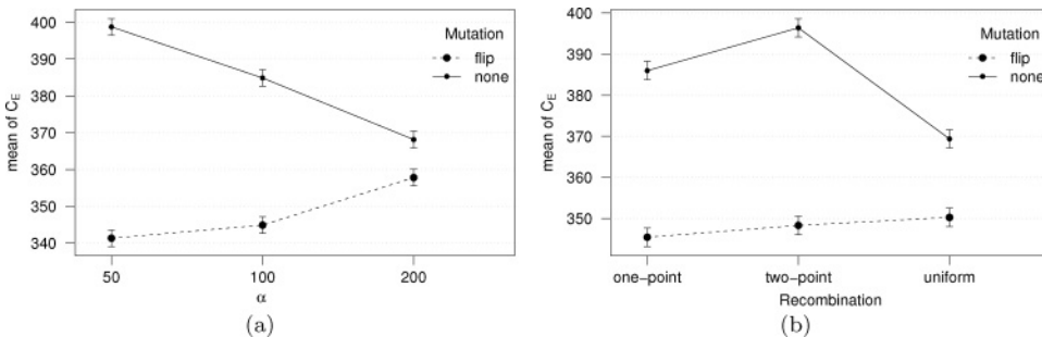
Figure 12: Interaction plots of SEA using the binary representation (the Vanzyl network). (a) Interaction between population size ( \alpha ) and mutation operator. (b) Interaction between recombination operator and mutation operator. The y axis gives the electricity cost ( C_E ).
