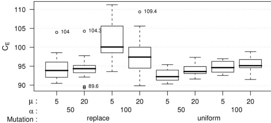
Figure 19: Boxplot of SEA using relative time-controlled triggers with rand-arithmetical recombination (the Richmond network). The y axis gives the electricity cost ( C_E ). The x axis denotes all possible combinations of parameter mutation, population size ( \alpha ), and parent/offspring population size ( \mu ) used in the runs summarised by each boxplot.
