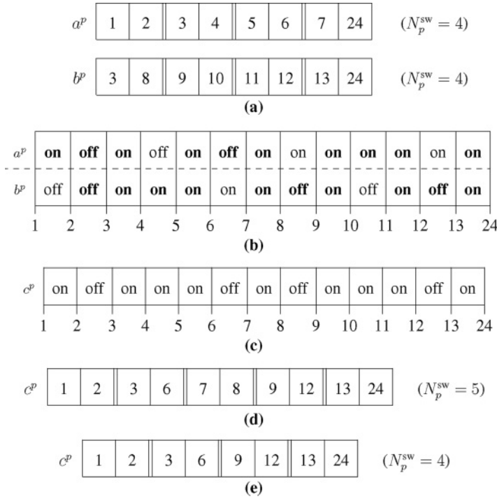
Figure 7: Example of uniform recombination for absolute time-controlled trigger representation.
