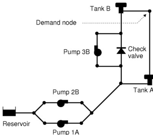
Figure 10: Vanzyl test network.
