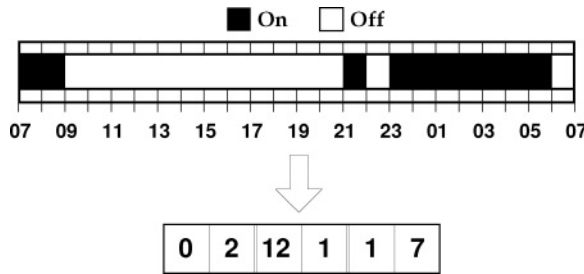
Figure 5: Example of relative time-controlled trigger representation.
