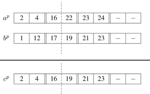
Figure 6: Example of one-point recombination for absolute time-controlled triggers.
