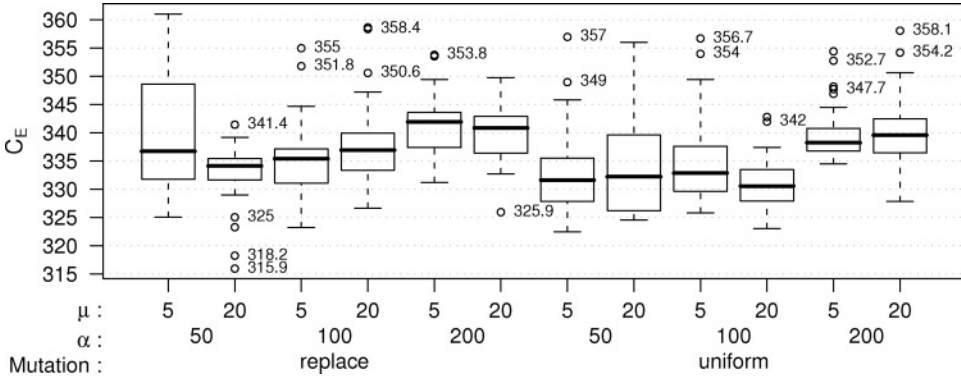
Figure 17: Boxplot of SEA with rand-arithmetical recombination using relative time-controlled triggers (the Vanzyt network). The y axis gives the electricity cost ( C_E ). The x axis denotes all possible combinations of parameter mutation, population size ( \alpha ), and parent/offspring population size ( \mu ) used in the runs summarised by each boxplot.
