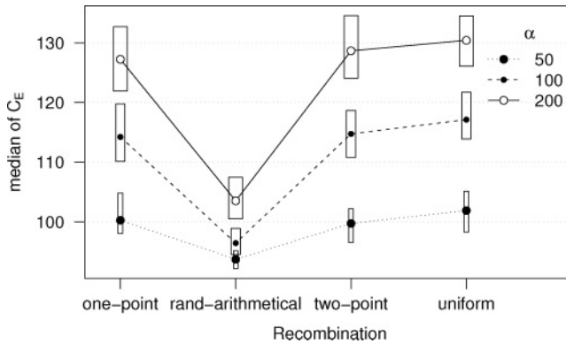
Figure 18: Boxplot of SEA using relative time-controlled triggers (the Richmond network). The y axis gives the electricity cost ( C_E ). The x axis denotes different recombinations. Points joined with a line denote runs using the same population size ( \alpha ).
